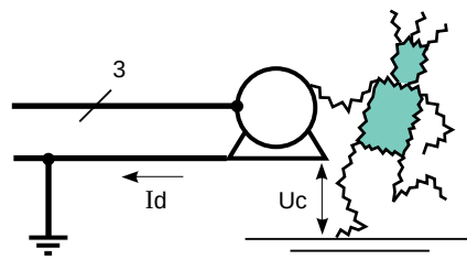
Fig. 3 : contacts directs et indirects.
